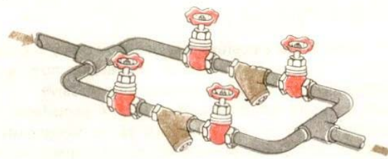
Figure. 1.1 Duplex Arrangement of Strainers in a Pipeline
